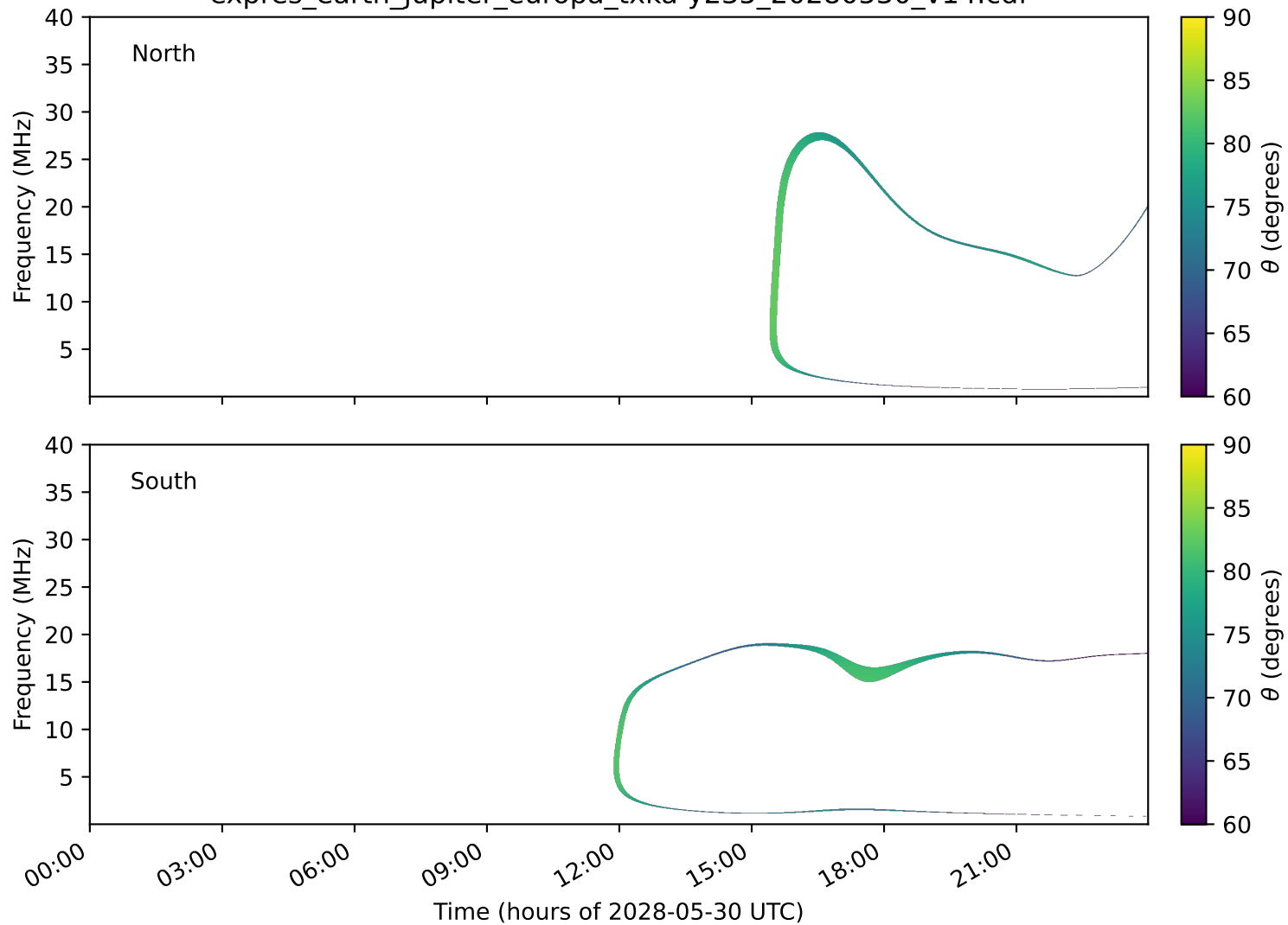
expres_earth_jupiter_europa_txka-y235_20280530_v14.cdf
