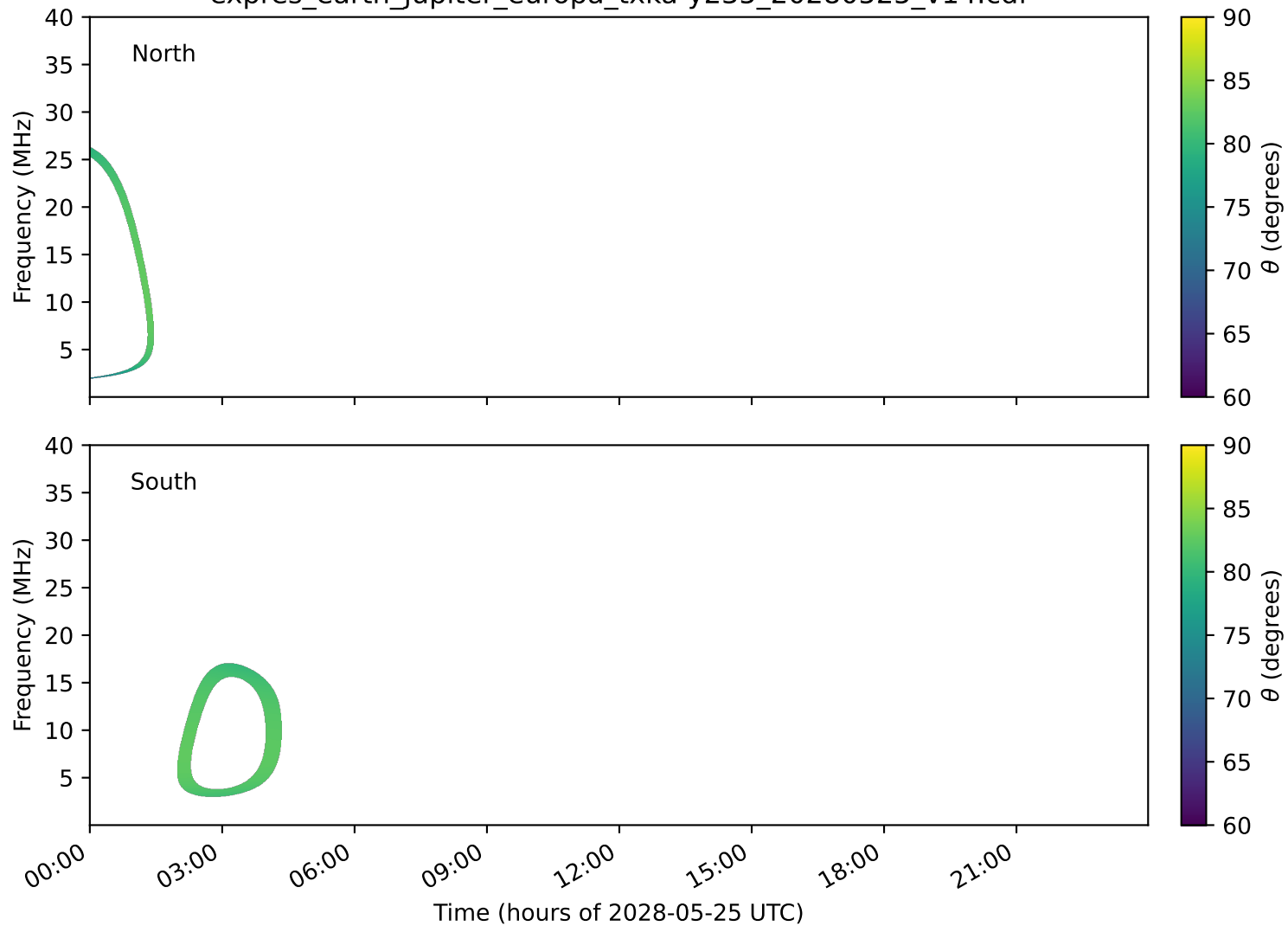
expres_earth_jupiter_europa_txka-y235_20280525_v14.cdf
