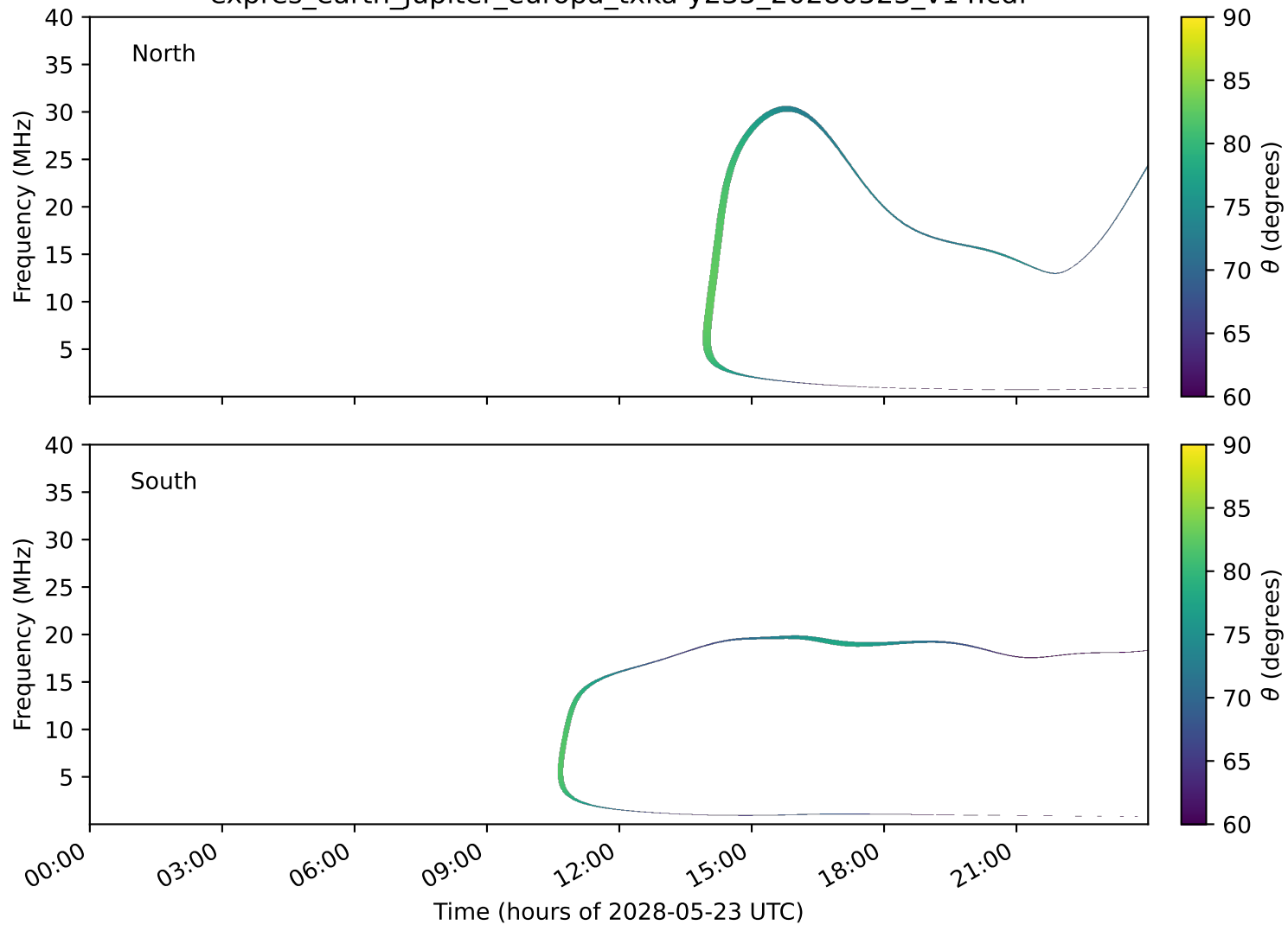
expres_earth_jupiter_europa_txka-y235_20280523_v14.cdf
