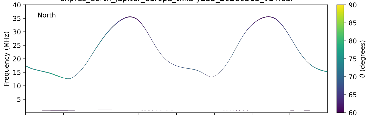
expres_earth_jupiter_europa_txka-y235_20280513_v14.cdf
