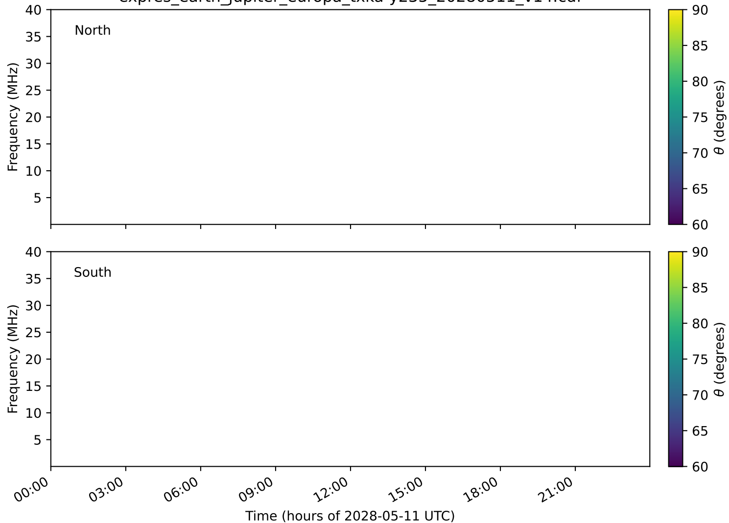
expres_earth_jupiter_europa_txka-y235_20280511_v14.cdf
