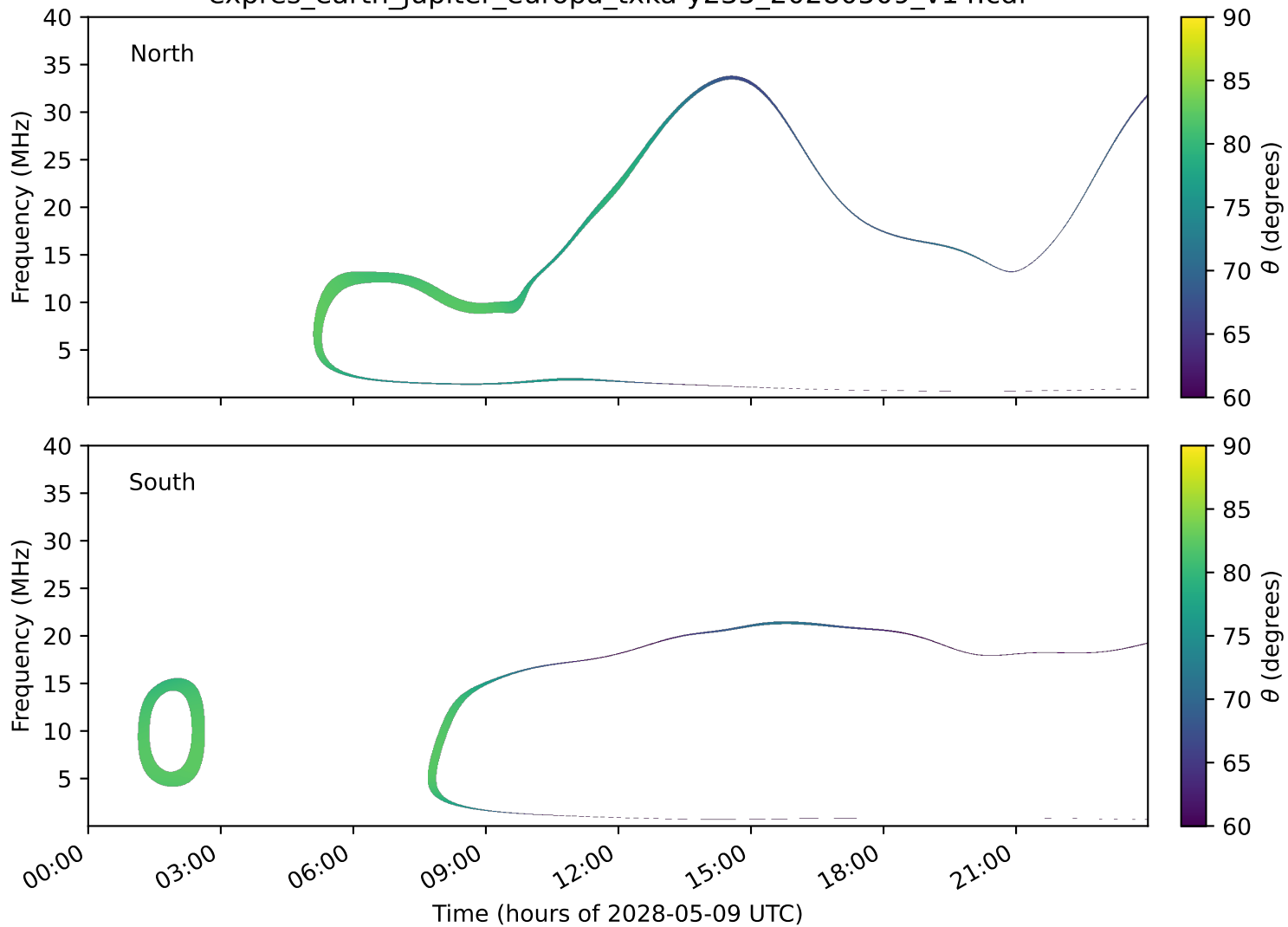
expres_earth_jupiter_europa_txka-y235_20280509_v14.cdf
