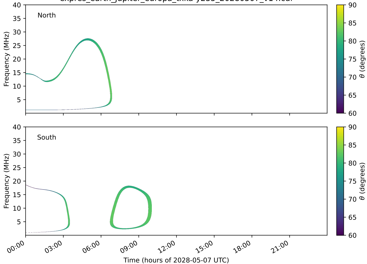
expres_earth_jupiter_europa_txka-y235_20280507_v14.cdf
