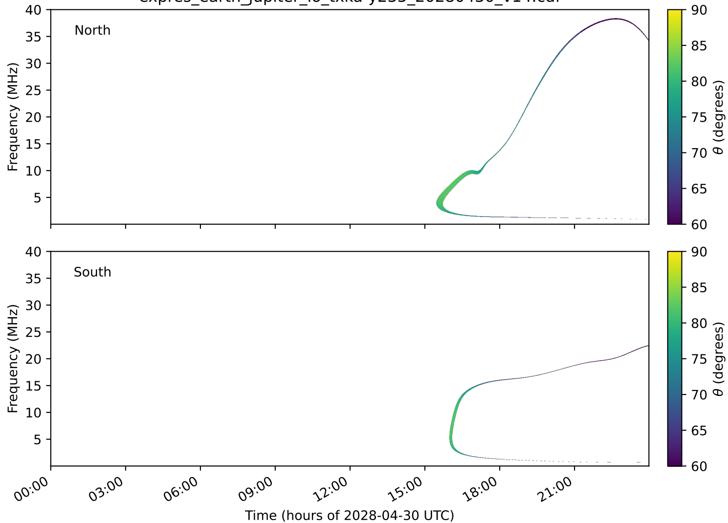
expres_earth_jupiter_io_txka-y235_20280430_v14.cdf
