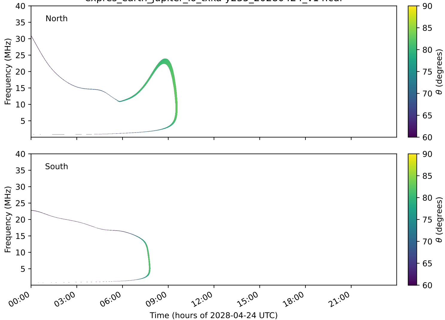
expres_earth_jupiter_io_txka-y235_20280424_v14.cdf
