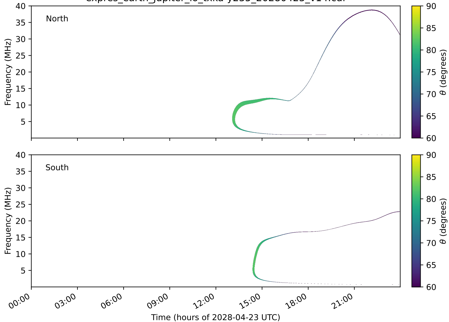
expres_earth_jupiter_io_txka-y235_20280423_v14.cdf
