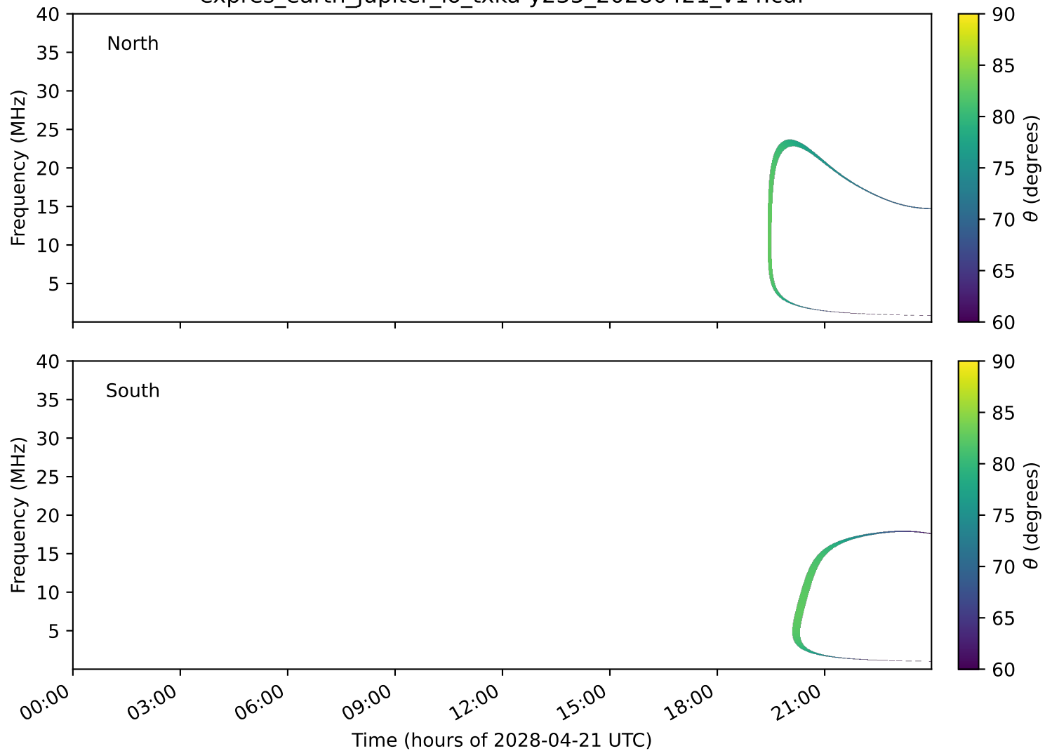
expres_earth_jupiter_io_txka-y235_20280421_v14.cdf
