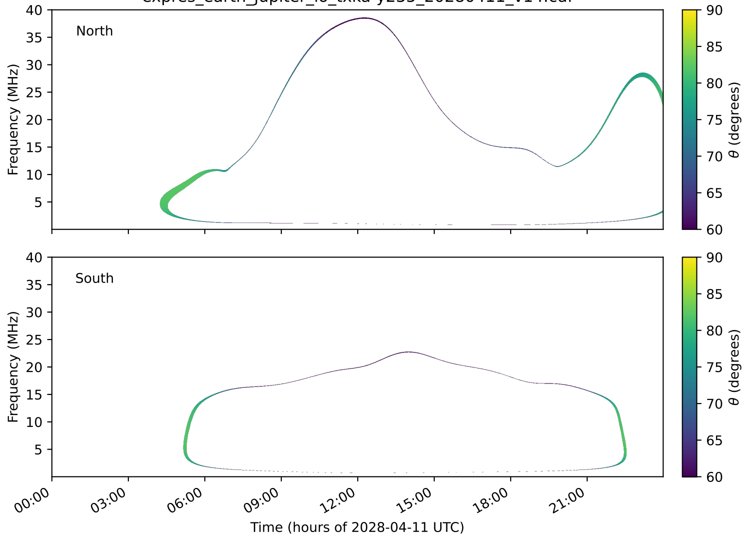
expres_earth_jupiter_io_txka-y235_20280411_v14.cdf
