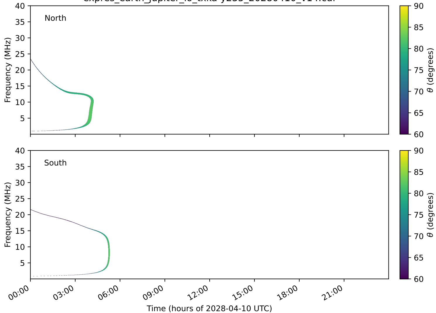
expres_earth_jupiter_io_txka-y235_20280410_v14.cdf
