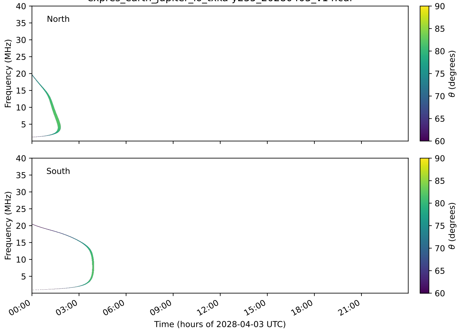
expres_earth_jupiter_io_txka-y235_20280403_v14.cdf
