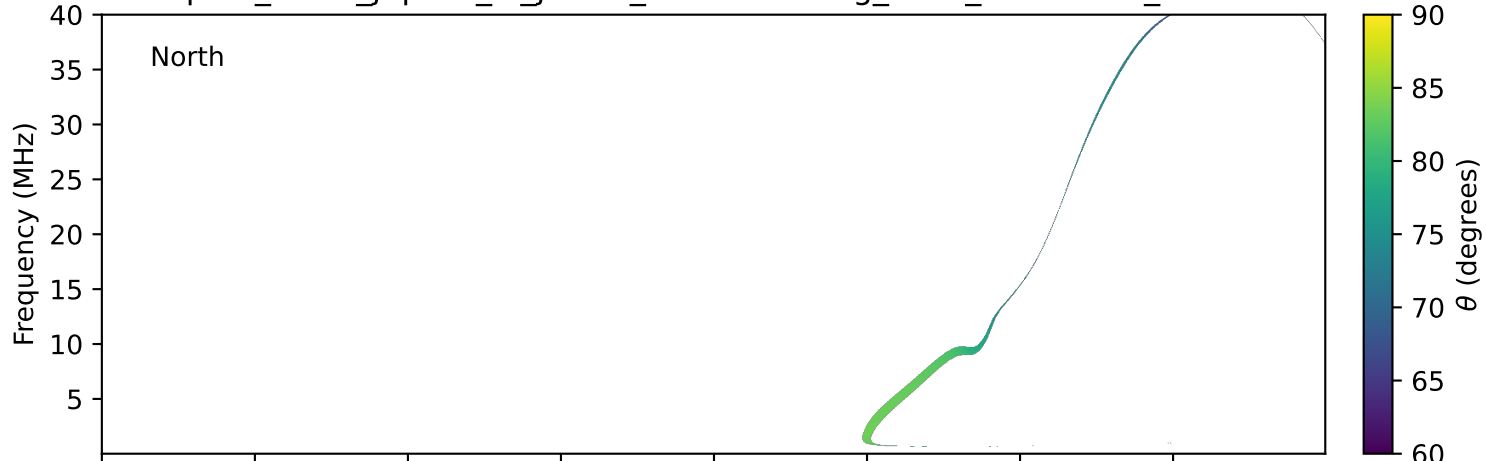
expres_earth_jupiter_io_jrm33_lossc-wid1deg_3kev_20280430_v11.cdf
