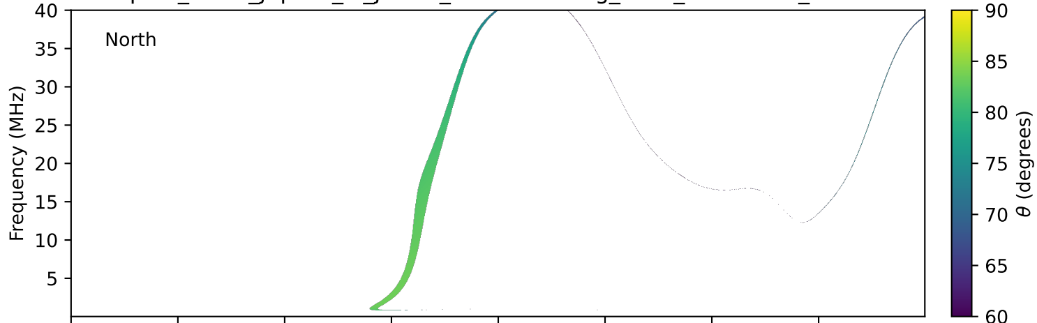
expres_earth_jupiter_io_jrm33_lossc-wid1deg_3kev_20280425_v11.cdf
