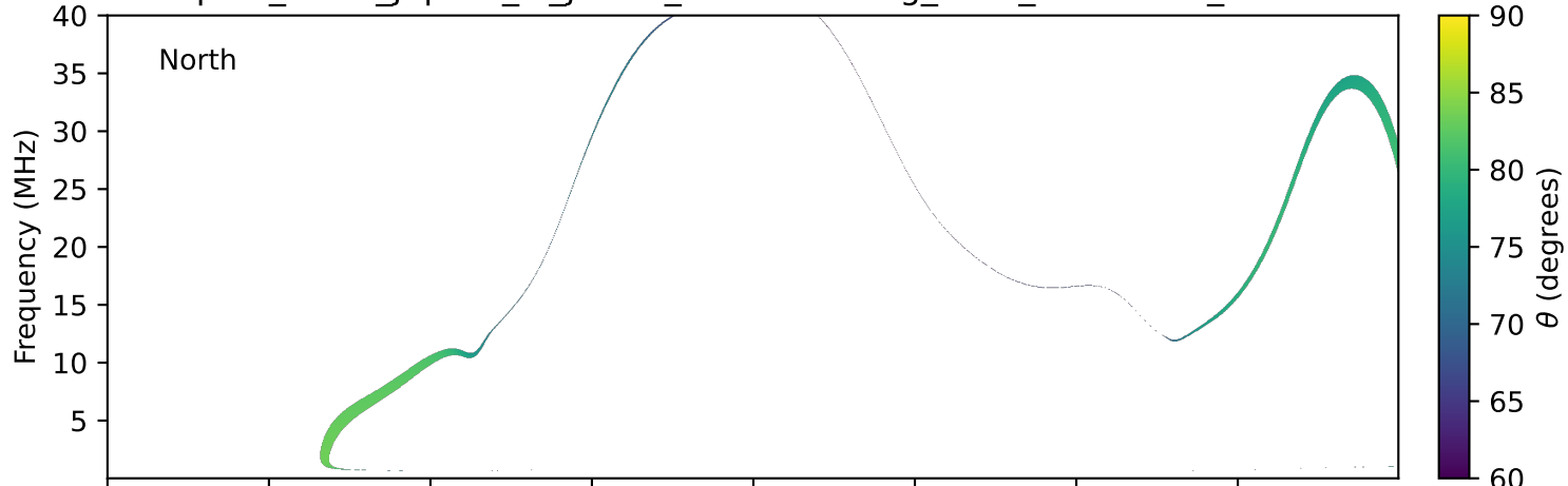
expres_earth_jupiter_io_jrm33_lossc-wid1deg_3kev_20280411_v11.cdf
