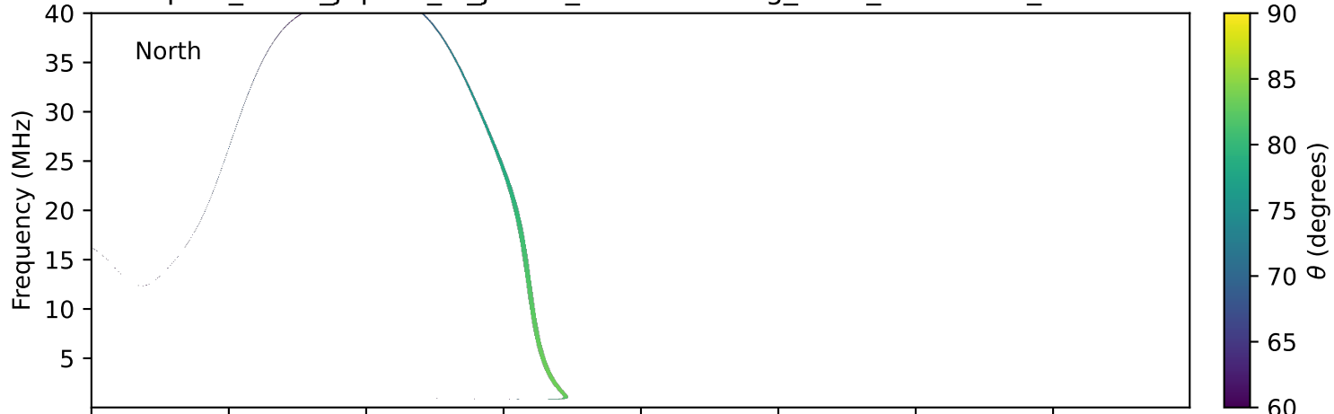
expres_earth_jupiter_io_jrm33_lossc-wid1deg_3kev_20280408_v11.cdf
