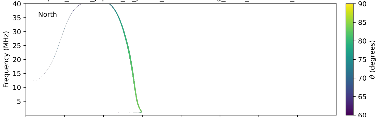
expres_earth_jupiter_io_jrm33_lossc-wid1deg_3kev_20280401_v11.cdf
