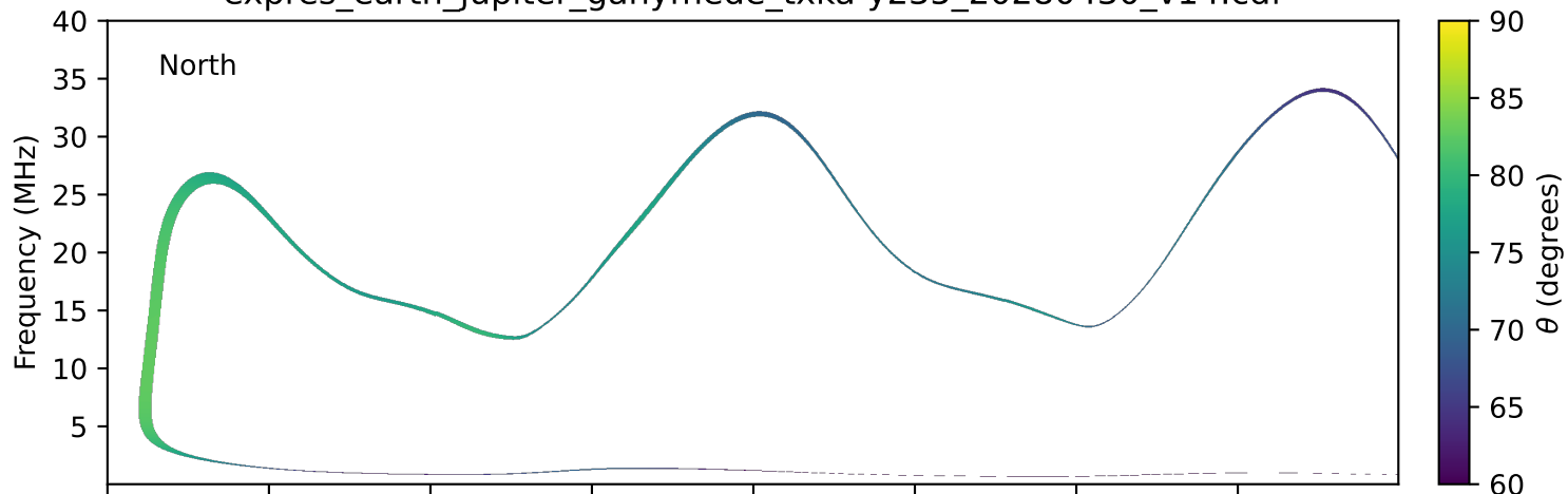
expres_earth_jupiter_ganymede_txka-y235_20280430_v14.cdf
