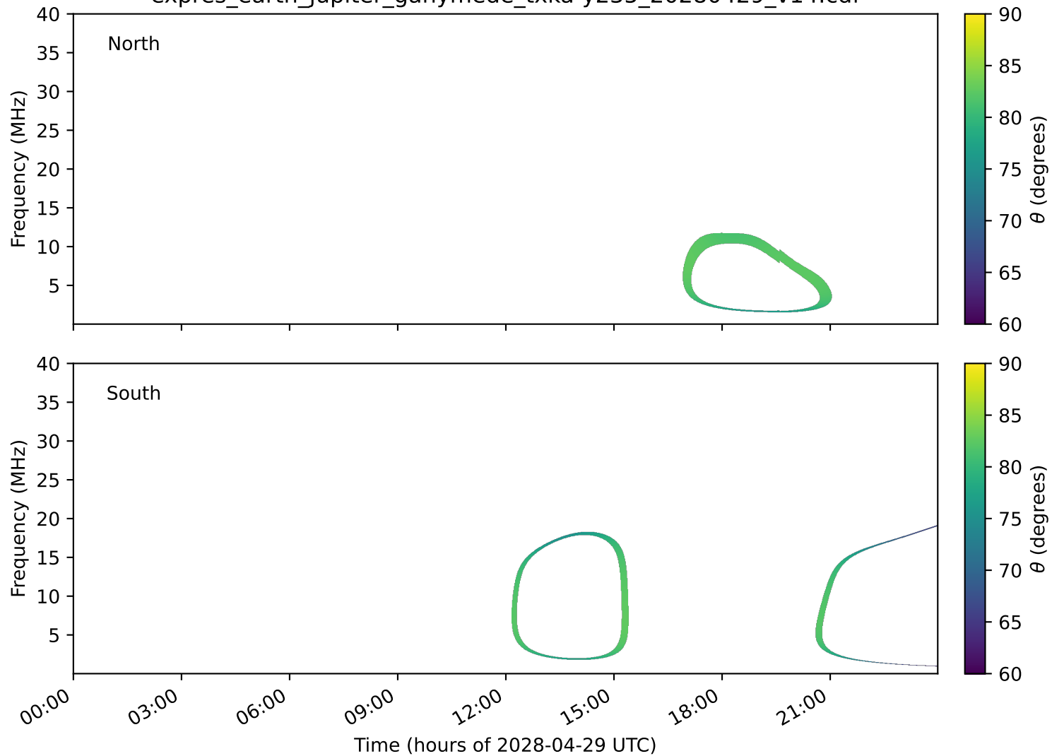
expres_earth_jupiter_ganymede_txka-y235_20280429_v14.cdf
