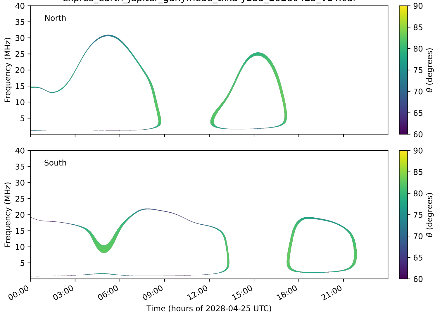
expres_earth_jupiter_ganymede_txka-y235_20280425_v14.cdf
