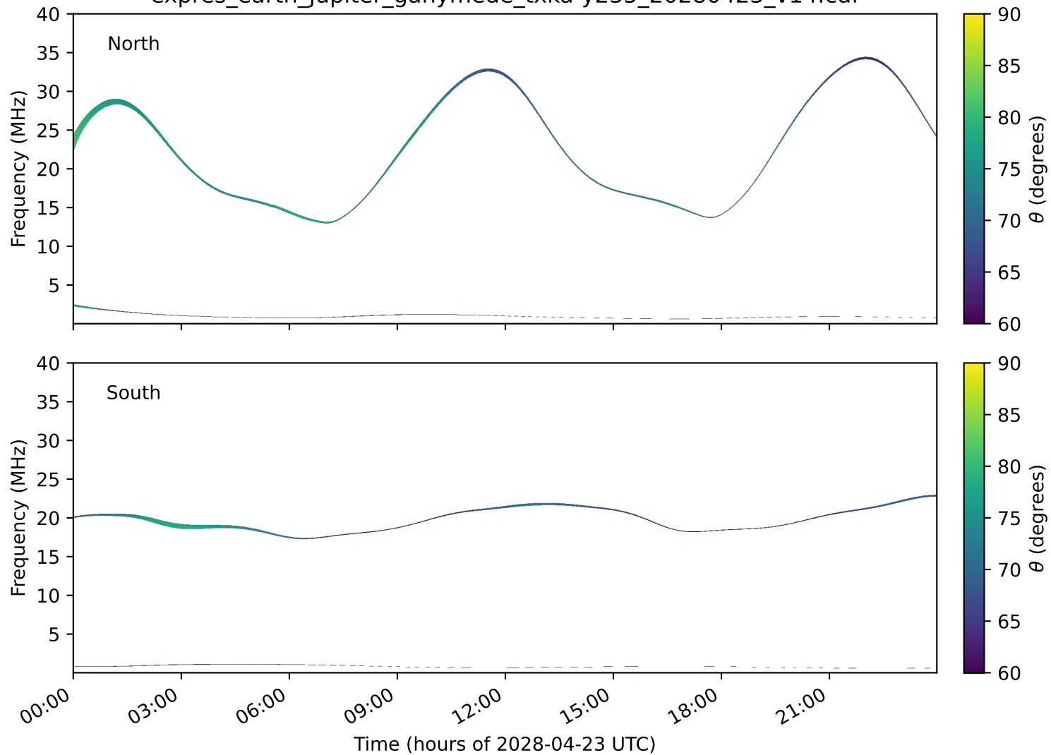
expres_earth_jupiter_ganymede_txka-y235_20280423_v14.cdf
