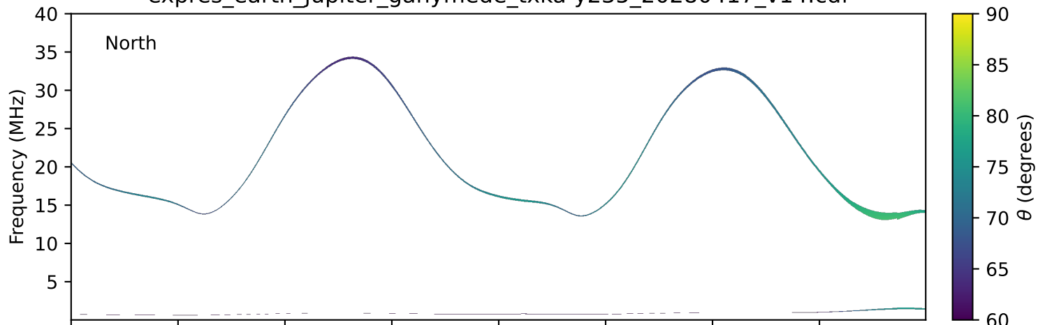
expres_earth_jupiter_ganymede_txka-y235_20280417_v14.cdf
