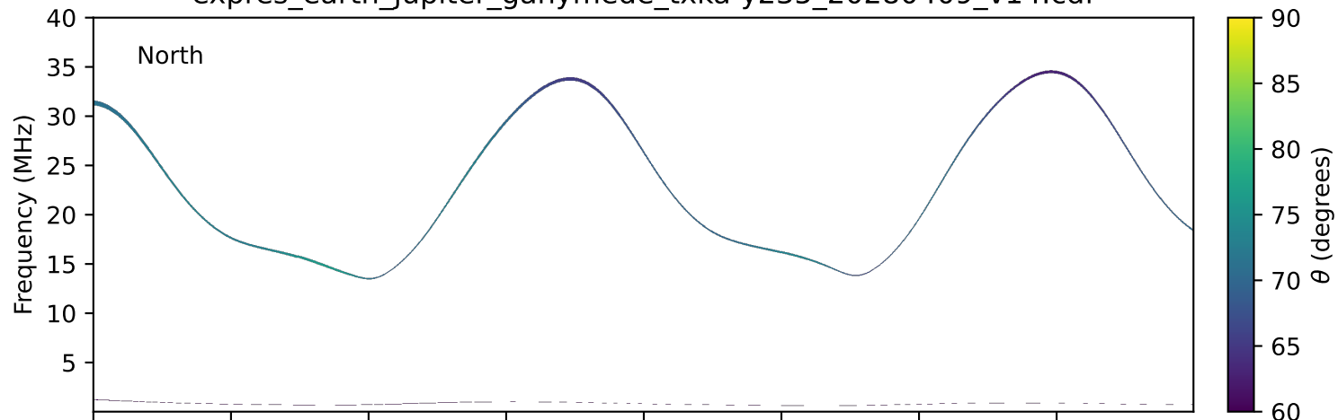
expres_earth_jupiter_ganymede_txka-y235_20280409_v14.cdf
