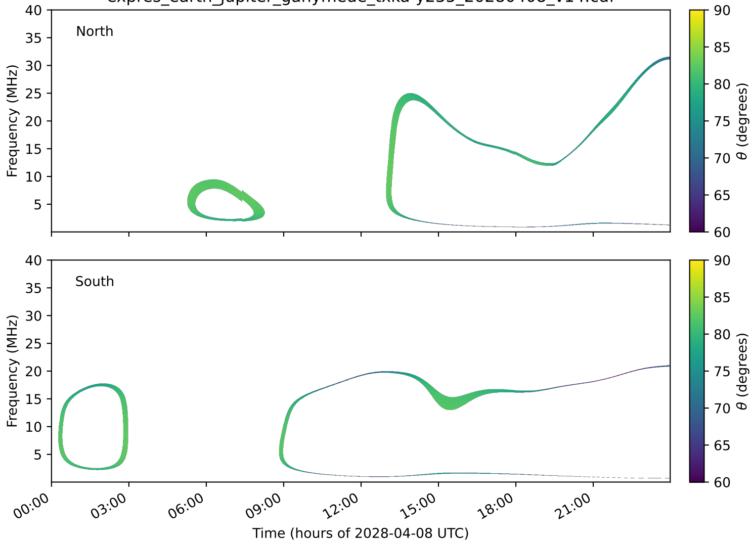
expres_earth_jupiter_ganymede_txka-y235_20280408_v14.cdf
