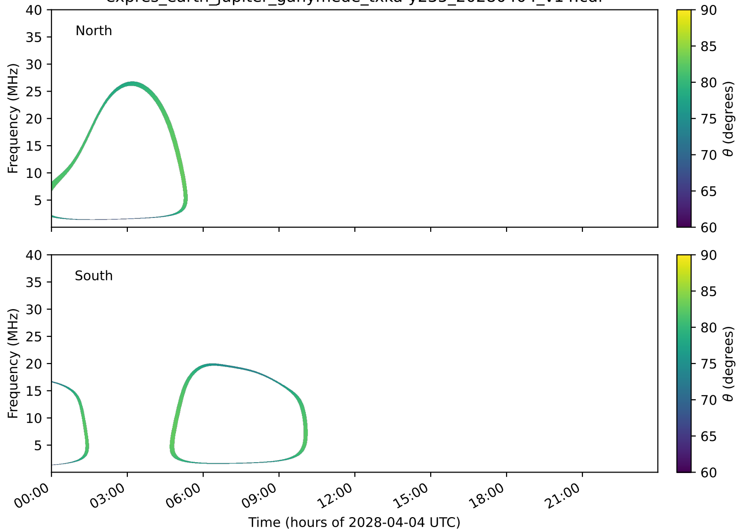
expres_earth_jupiter_ganymede_txka-y235_20280404_v14.cdf
