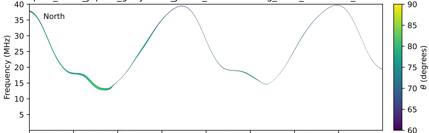
expres_earth_jupiter_ganymede_jrm33_lossc-wid1deg_3kev_20280409_v11.cdf
