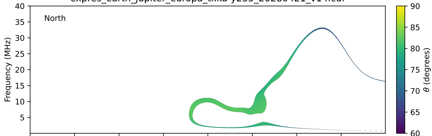
expres_earth_jupiter_europa_txka-y235_20280421_v14.cdf
