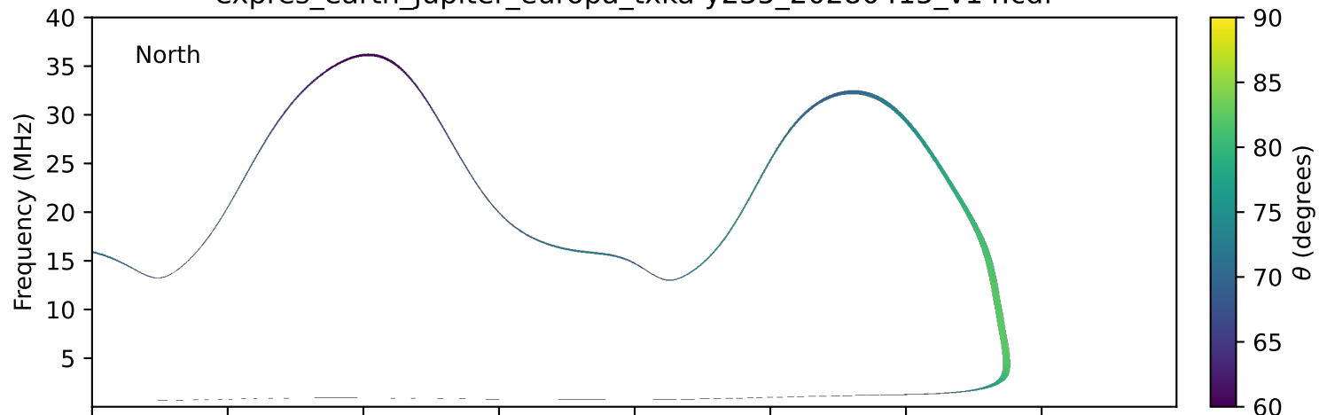
expres_earth_jupiter_europa_txka-y235_20280415_v14.cdf
