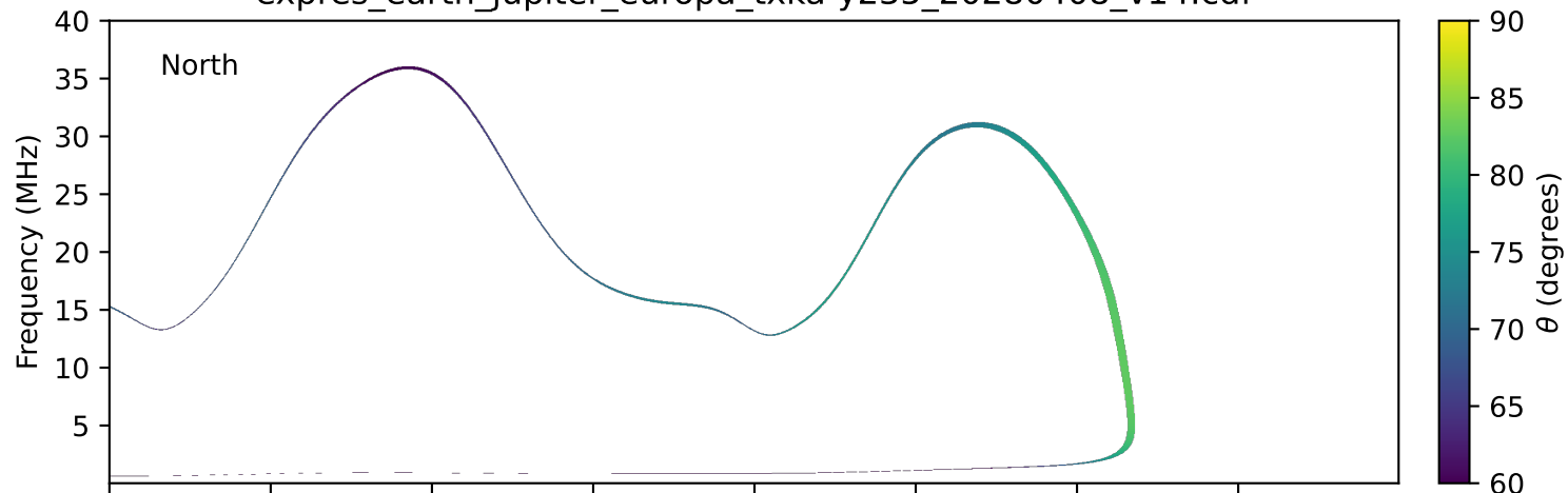
expres_earth_jupiter_europa_txka-y235_20280408_v14.cdf
