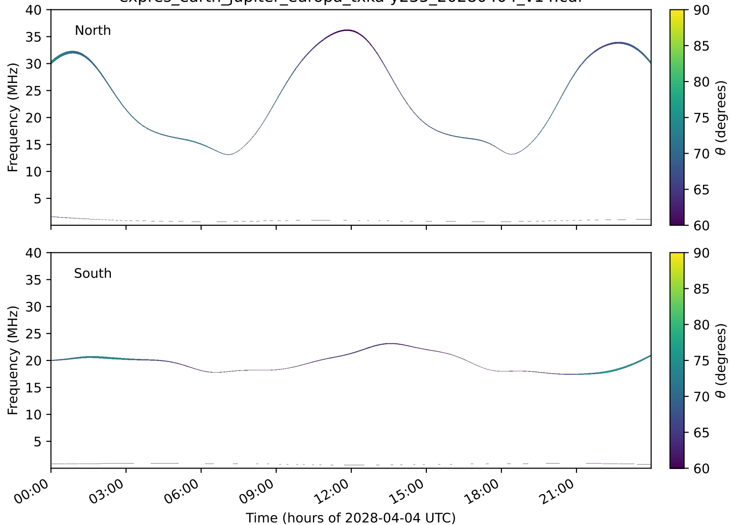
expres_earth_jupiter_europa_txka-y235_20280404_v14.cdf
