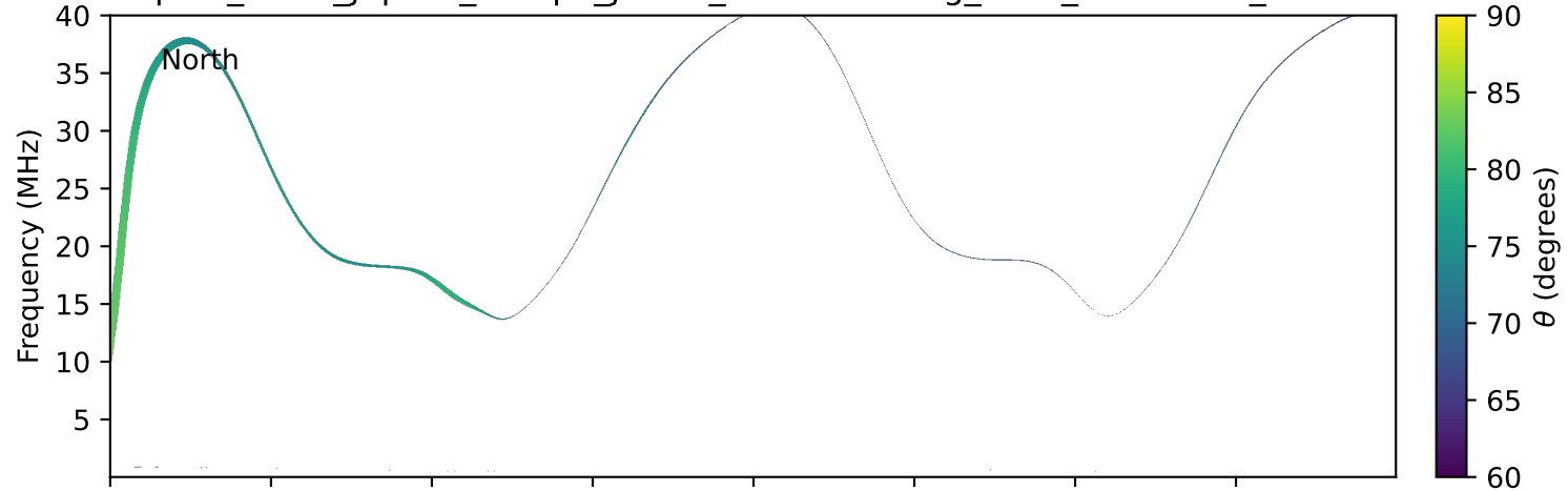
expres_earth_jupiter_europa_jrm33_lossc-wid1deg_3kev_20280411_v11.cdf
