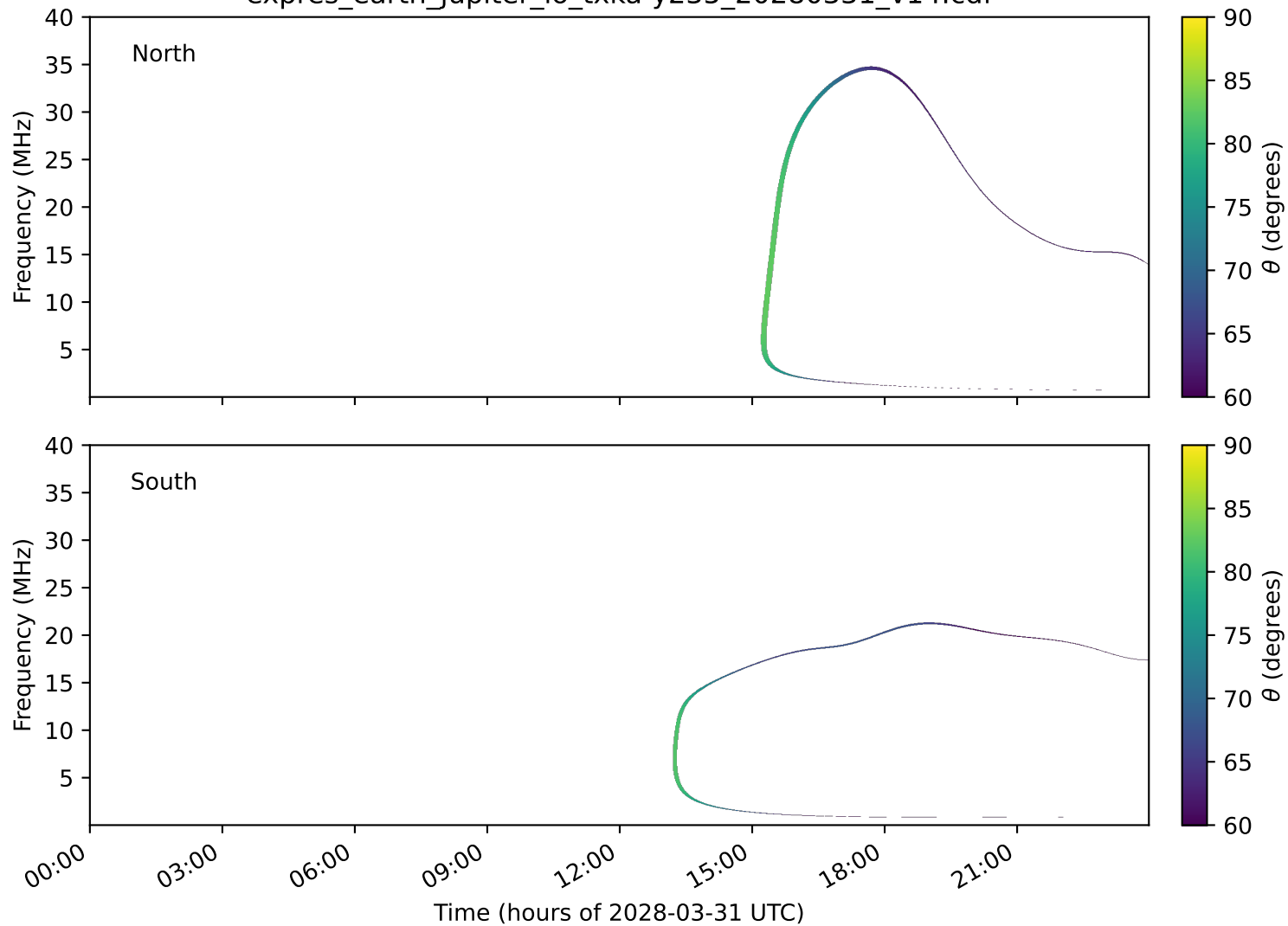
expres_earth_jupiter_io_txka-y235_20280331_v14.cdf
