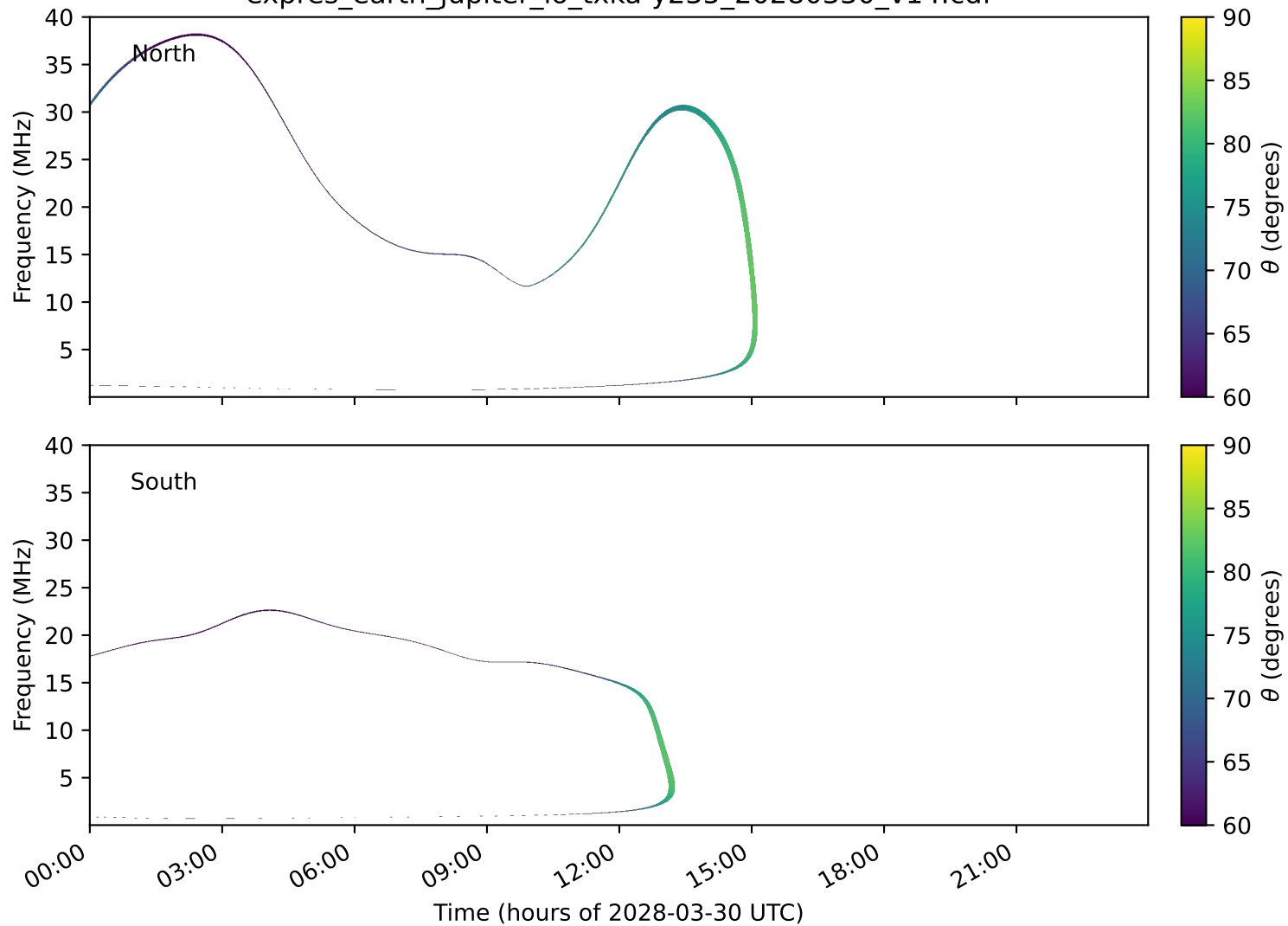
expres_earth_jupiter_io_txka-y235_20280330_v14.cdf
