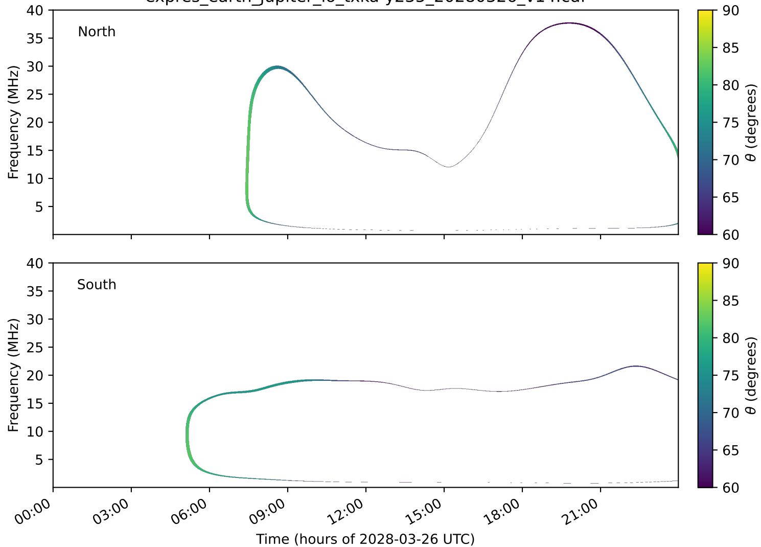
expres_earth_jupiter_io_txka-y235_20280326_v14.cdf
