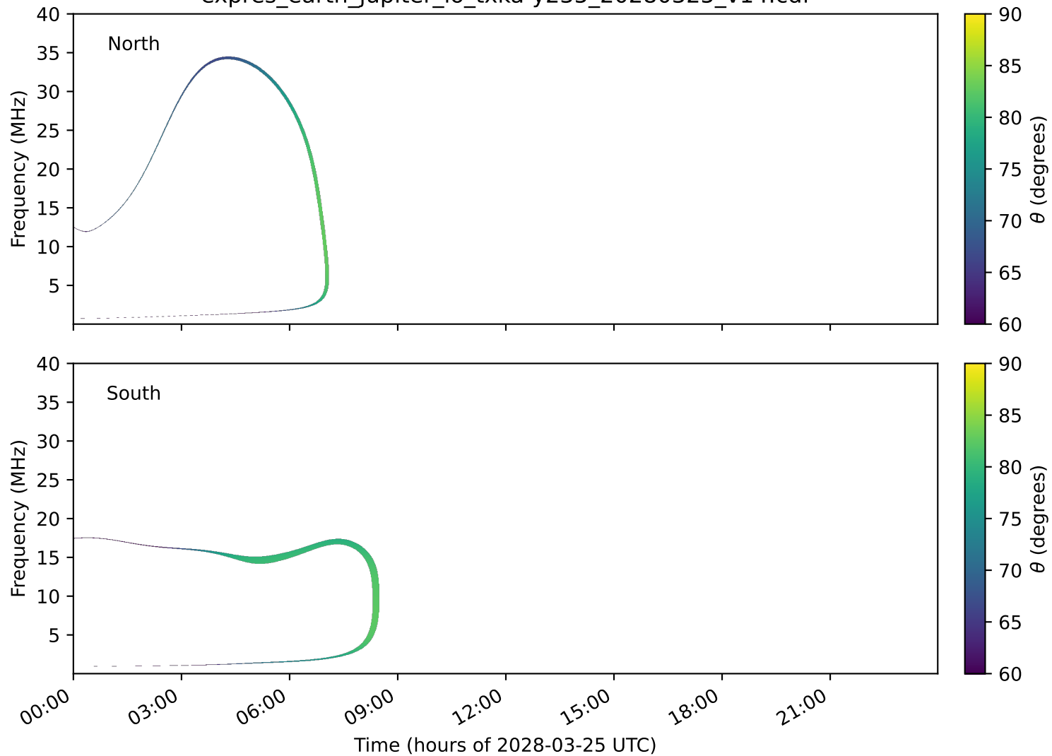
expres_earth_jupiter_io_txka-y235_20280325_v14.cdf
