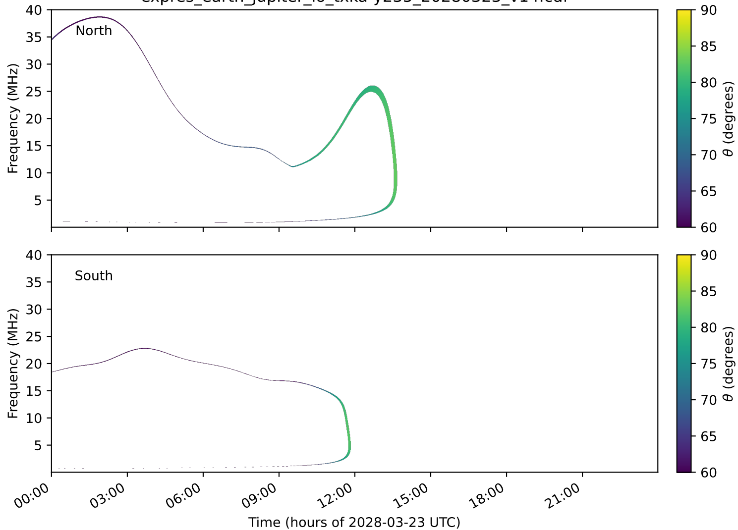
expres_earth_jupiter_io_txka-y235_20280323_v14.cdf
