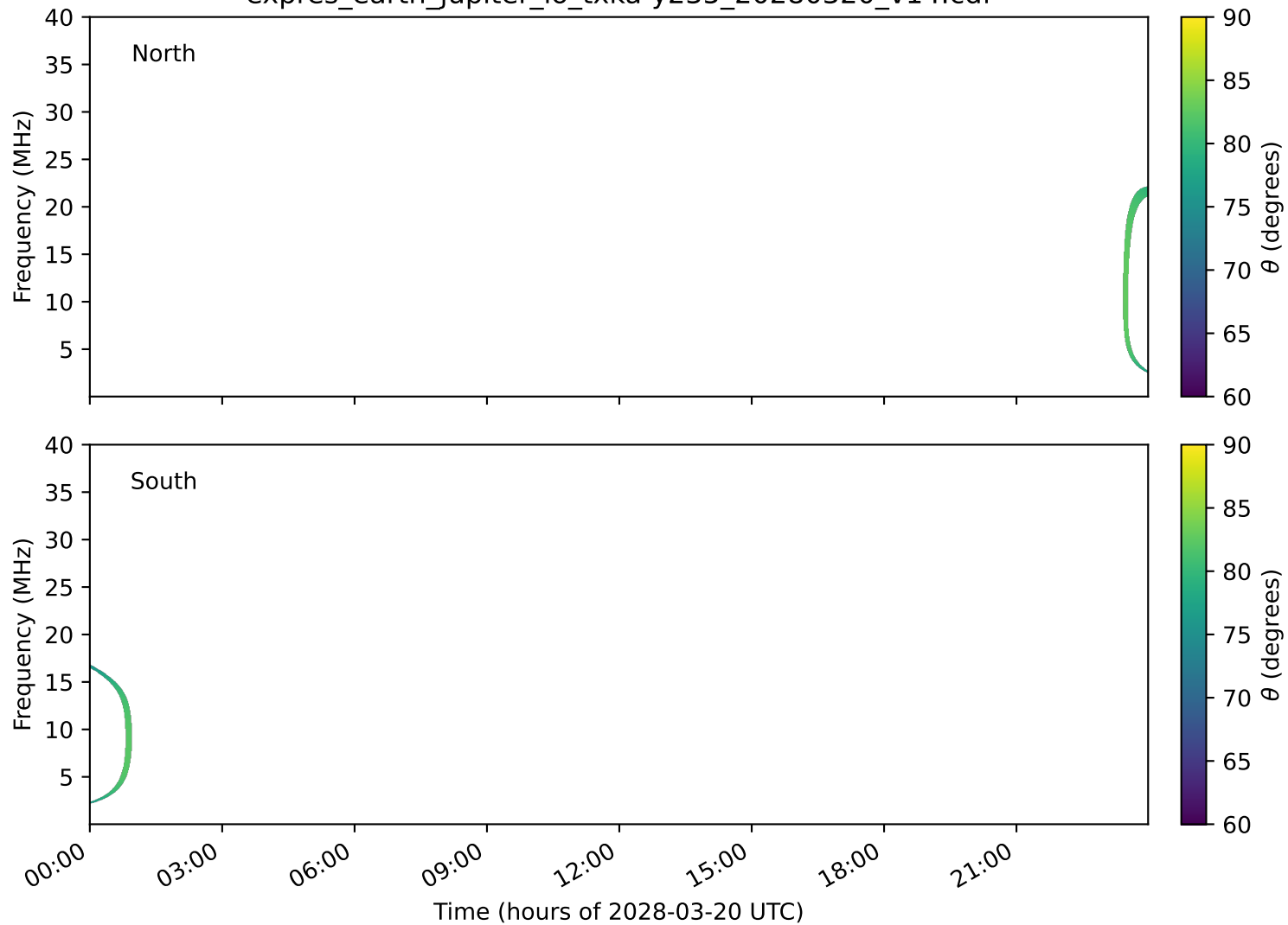
expres_earth_jupiter_io_txka-y235_20280320_v14.cdf
