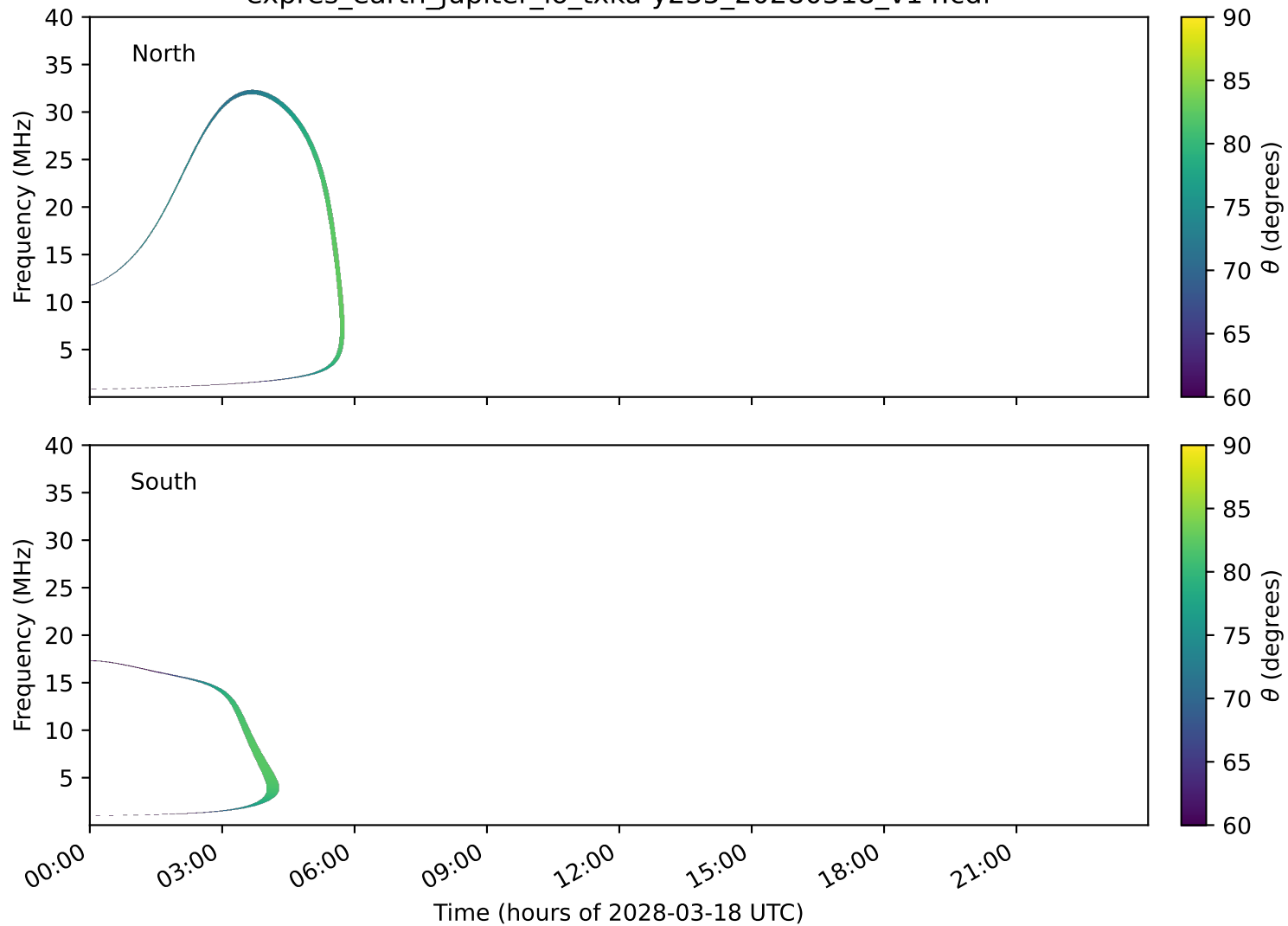
expres_earth_jupiter_io_txka-y235_20280318_v14.cdf
