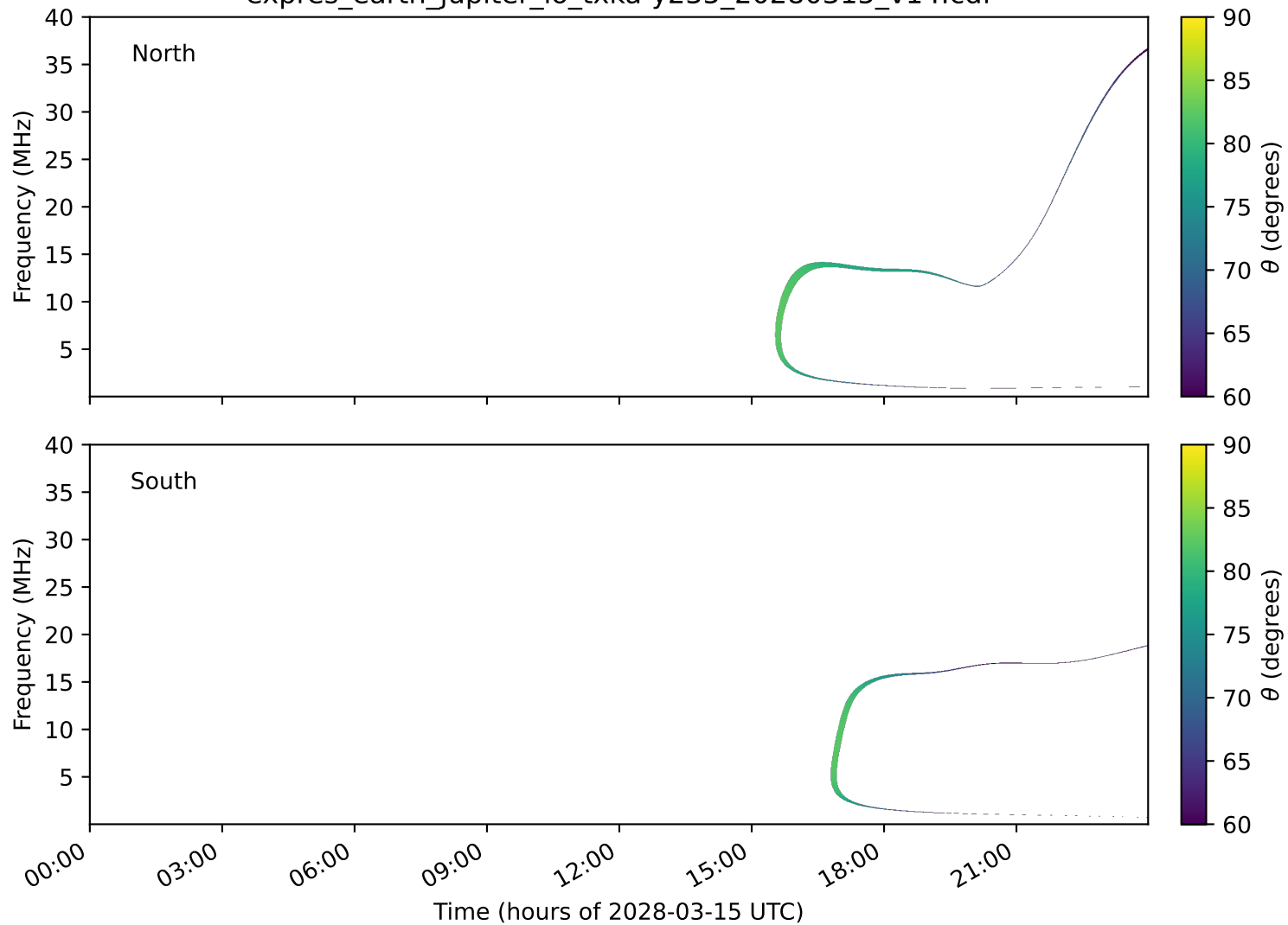
expres_earth_jupiter_io_txka-y235_20280315_v14.cdf
