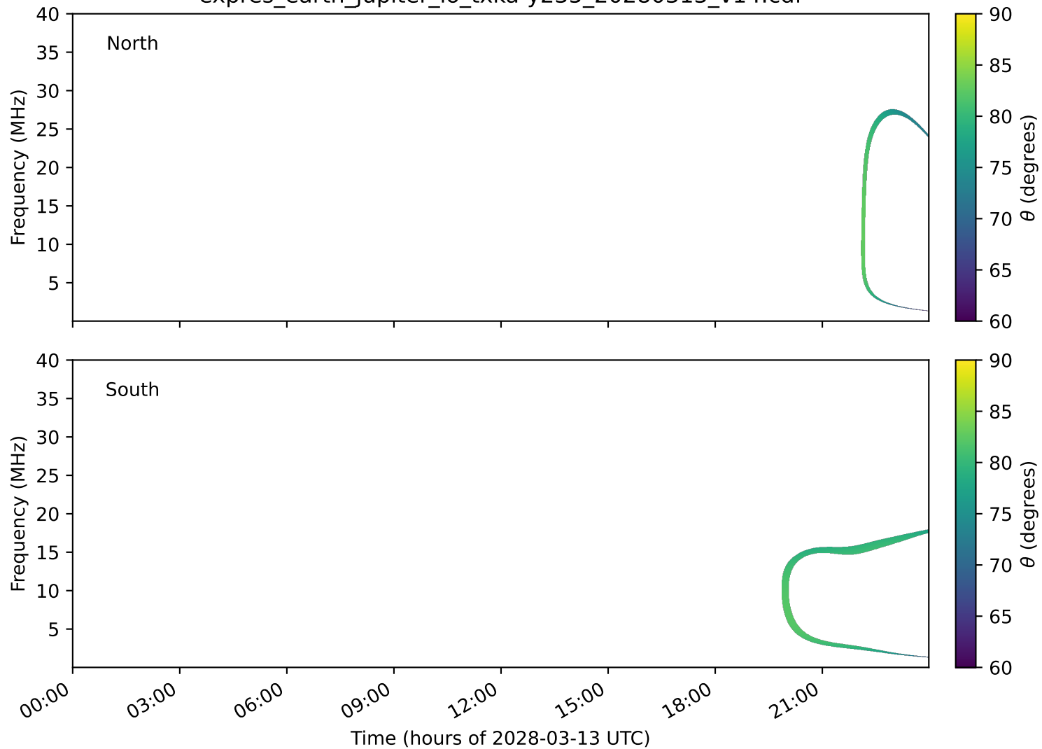
expres_earth_jupiter_io_txka-y235_20280313_v14.cdf
