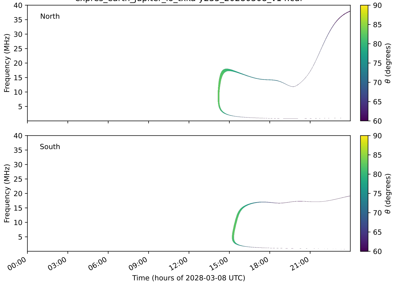
expres_earth_jupiter_io_txka-y235_20280308_v14.cdf
