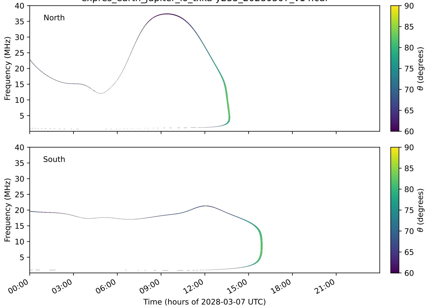
expres_earth_jupiter_io_txka-y235_20280307_v14.cdf
