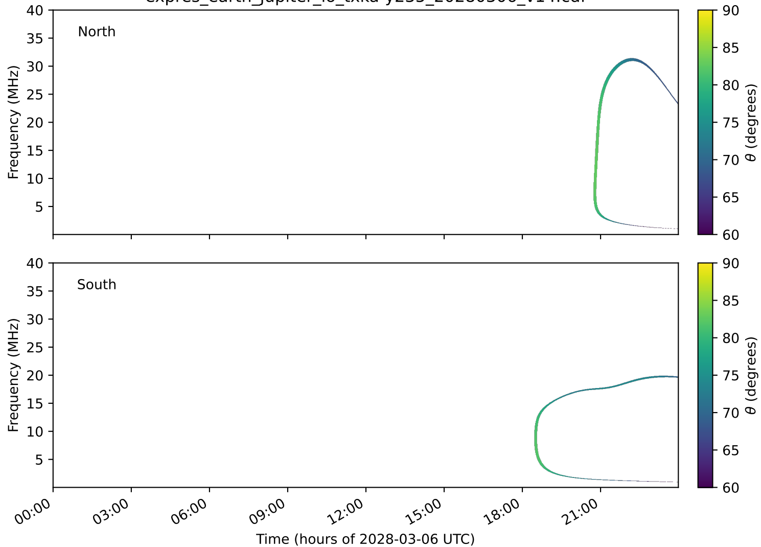
expres_earth_jupiter_io_txka-y235_20280306_v14.cdf
