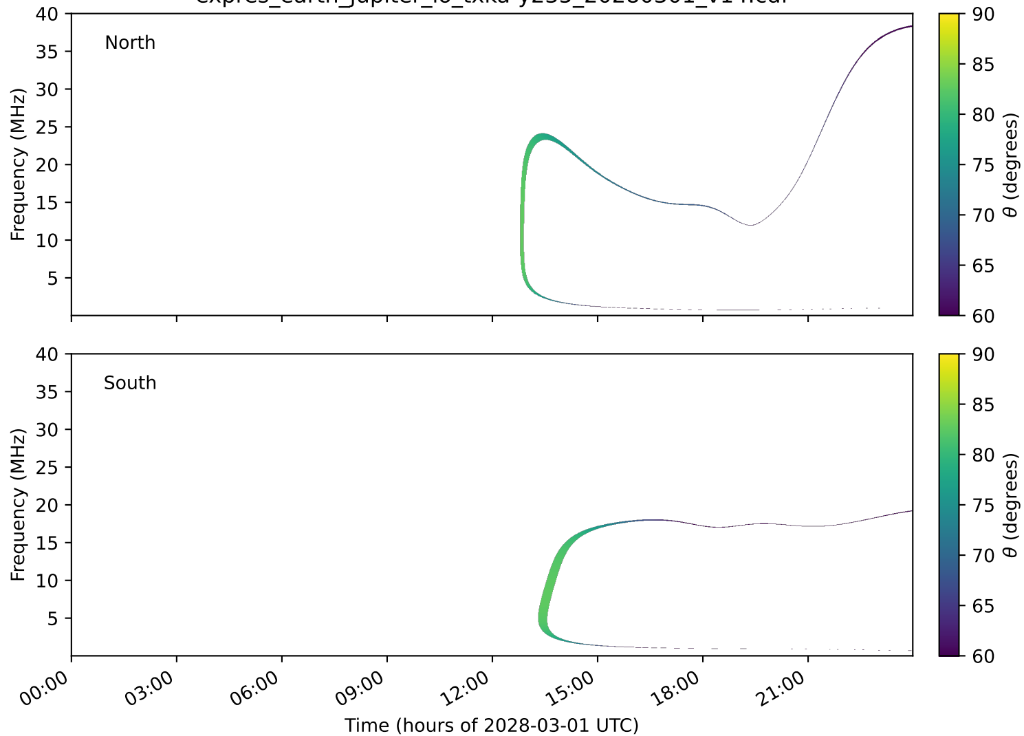
expres_earth_jupiter_io_txka-y235_20280301_v14.cdf
