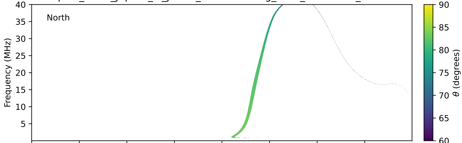
expres_earth_jupiter_io_jrm33_lossc-wid1deg_3kev_20280324_v11.cdf
