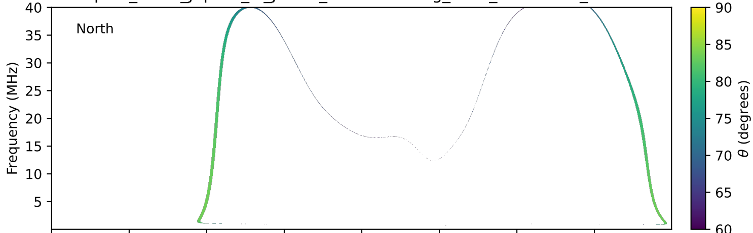
expres_earth_jupiter_io_jrm33_lossc-wid1deg_3kev_20280319_v11.cdf
