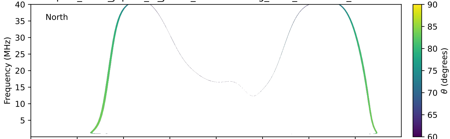
expres_earth_jupiter_io_jrm33_lossc-wid1deg_3kev_20280312_v11.cdf
