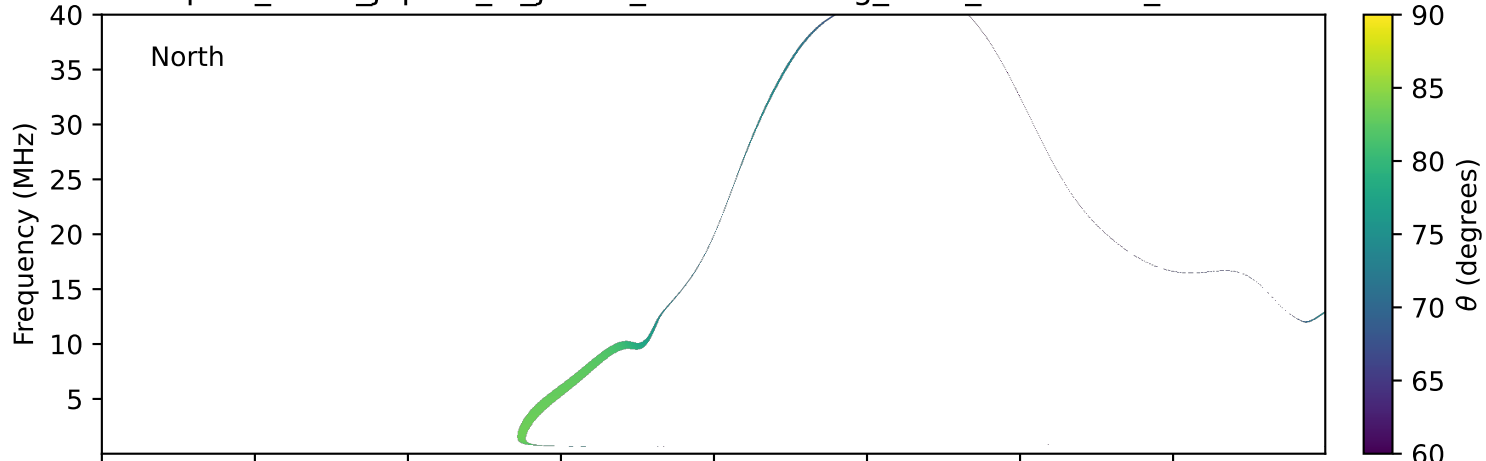
expres_earth_jupiter_io_jrm33_lossc-wid1deg_3kev_20280310_v11.cdf
